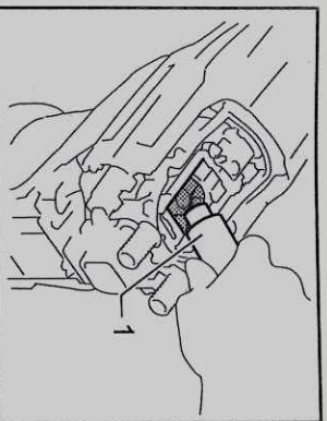
1. Hammer grease
