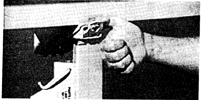
8. Mount the cradle on top of the telescoping section. Flip out the tilt latch to allow the cradle to tilt for loading and for hanging dry-wall on sidewalls and sloped ceilings.
