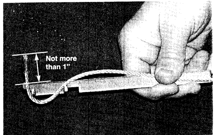
9. Load the cable installation tool as shown. To ease the installation procedure, there should not be more than 1" of cable extending at the end.
