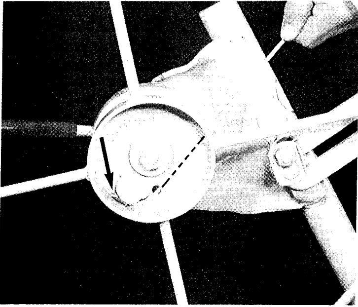
24. Feed the copper crimped end of the cable through the winch drum and secure it behind the mooring tab by hand pulling the cable snug as shown.
