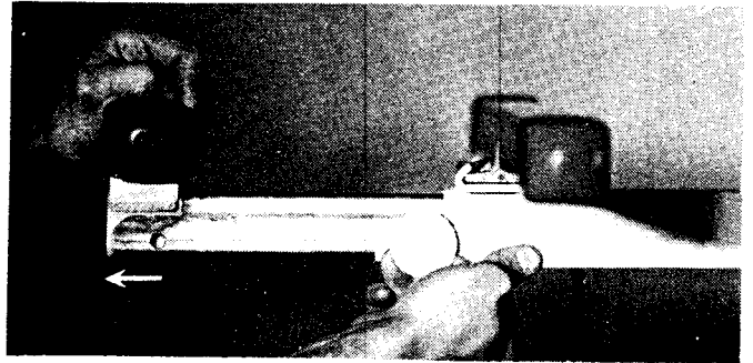
10. To extend the outriggers for use, pull out on the outrigger lock pin with your right hand and slide the outrigger out with your left hand as shown. The lock pin will engage at three different points on the outrigger: fully retracted, extended 21", or extended 33". MAKE SURE that the lock pins are engaged in one of these three positions before loading the unit. DO NOT use the PANELLIFT® with the outriggers extended beyond the 33" point. Retract the outriggers when storing or transporting the unit.
