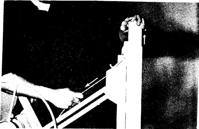
2. Pinch the two telescoping sections together and lift them out as a unit. Pulling the cable will help to raise them.
