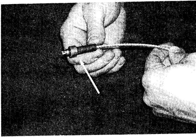
6. Make sure the rubber sleeve is seated completely against the anchoring bushing in the new cable.
