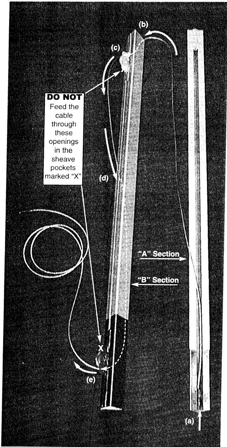
19. A correctly strung cable is shown above : Through the "A" section anchoring "V" from the bottom (a), into the top of the "B" section (b), back out through the sheave pocket at the end nearest the top of the telescoping section (c), into the slot of the "B" section (d), and out a final time through the end of the sheave pocket nearest the bottom of the "B" section (e).
