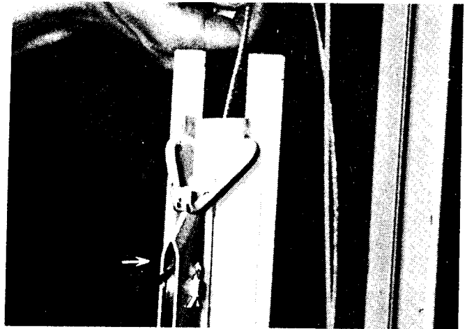
4. Feed the crimped end of the 186-00 cable through the frame sheave pocket from the top. It is VERY IMPORTANT that the cable passes OVER THE TOP of the brass sheave as shown here.
