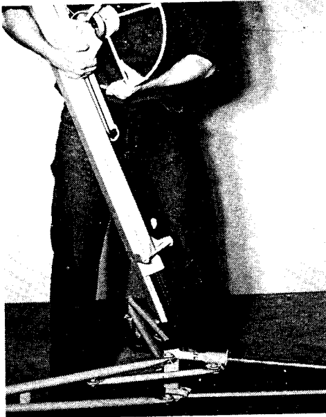
2A. Place the frame assembly on the tripod base.
