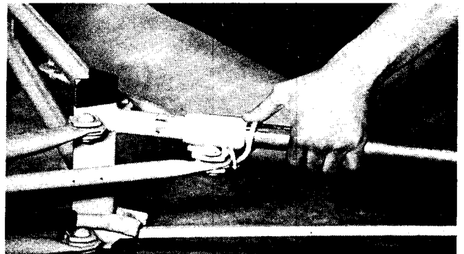
10. To collapse the tripod base, press down on the slide yoke ring and swing the legs in until they lock in the closed position.
