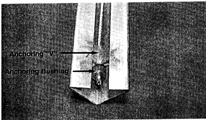
8. Pull the cable all the way through until the rubber sleeve passes under the anchoring "V" and the anchoring bushing sits tightly against the "V". WARNING!! DO NOT use a hammer to pound this assembly in place and DO NOT use a wedge or any other anchoring device. Doing so may damage the steel ball crimp and may cause the cable to fail under a load, possibly resulting in serious property damage, serious bodily injury, and/or death.
