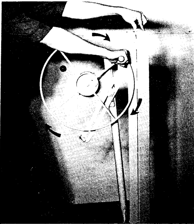
8. Hold the retaining hook in this position with your left hand and rotate the winch forward with your right hand. This will cause the winch assembly to fold up against the frame. When the slide bar contacts the frame, tighten the cable just sufficiently to hold the winch in the collapsed position.
