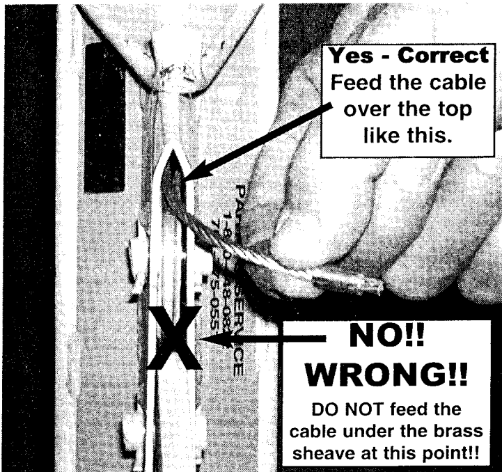
22. MAKE SURE that the cable feeds over the TOP of the brass sheave as shown in steps 21 and 22.
