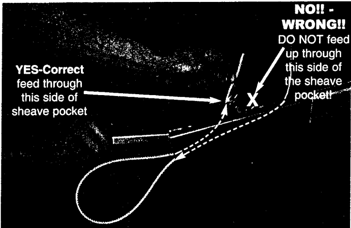
17. Repeat the process performed in steps 11 and 12: Insert the crimped end of the cable up into the end of the sheave pocket at the end nearest the end of the "B" section as traced by the dotted arrows. With a motion like that of tightening a screw driver, twist the installation tool while holding the copper crimped end of the cable up into the sheave pocket. The cable will pop loose from the tool and up through the sheave pocket. Pull the crimped end out completely to remove the slack.
