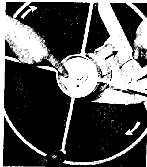
6. Feed the cable through the winch drum and secure it firmly behind the mooring tab as shown. Rotate the winch wheel in the direction indicated to take up the slack in the cable.
