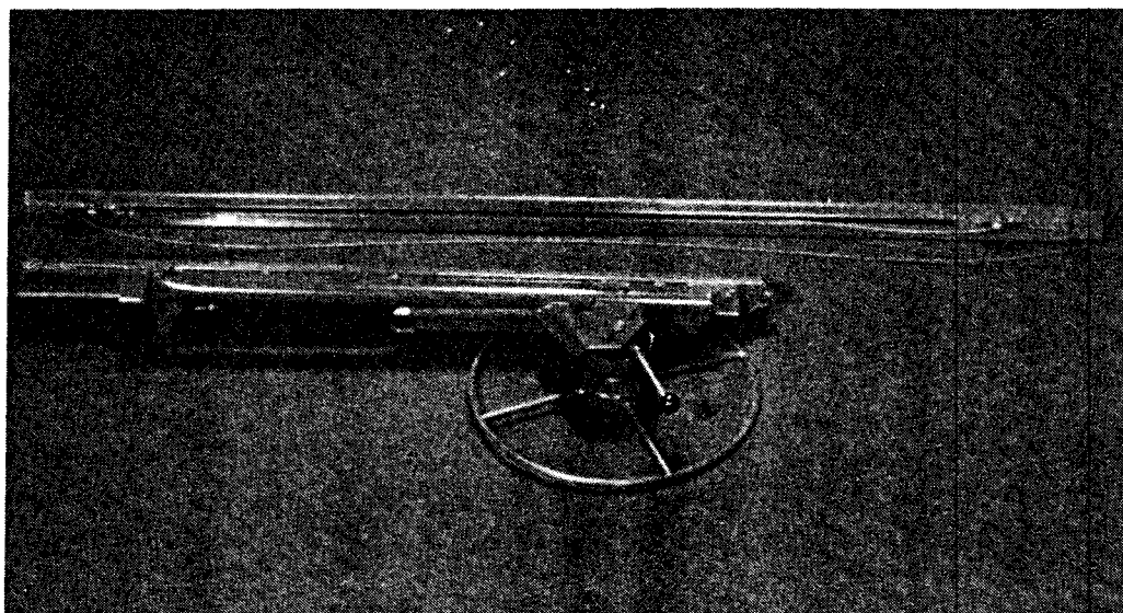
The extension 186-00 consists of two 6' telescoping sections and allows the PANELLIFT® Drywall Lift to reach 15 feet. This unit easily interchanges with the standard 4' telescoping sections shown here for comparison.
