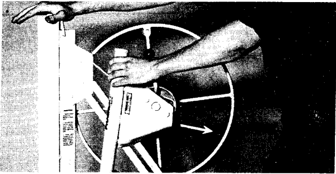
5. Place your right hand on top of the frame and pull the winch assembly towards you. While pulling the winch towards you, grip the brake arm sufficiently to prevent back-lash of the cable on the winch.
