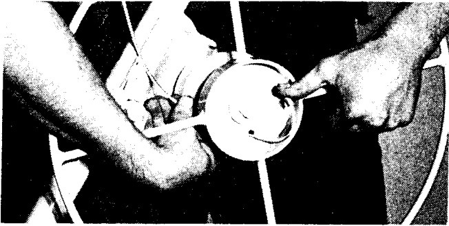
1. Loosen the cable from the mooring tab on the winch and pull it out through the winch drum.
