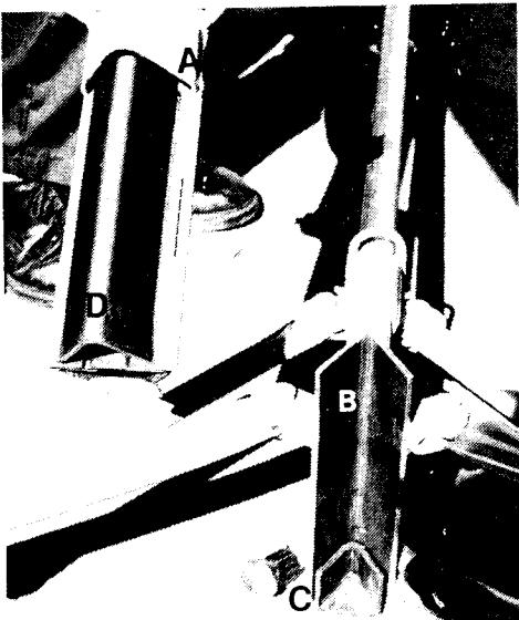
2B. Pocket "A" slides OVER angle "B" while angle "C" slides INSIDE angle "D".
