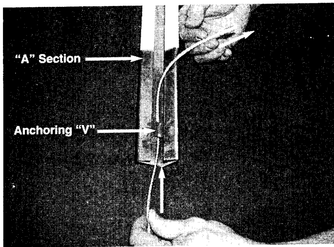
7. Feed the copper crimped end of the cable through the "A" section anchoring "V" from the bottom as shown.
