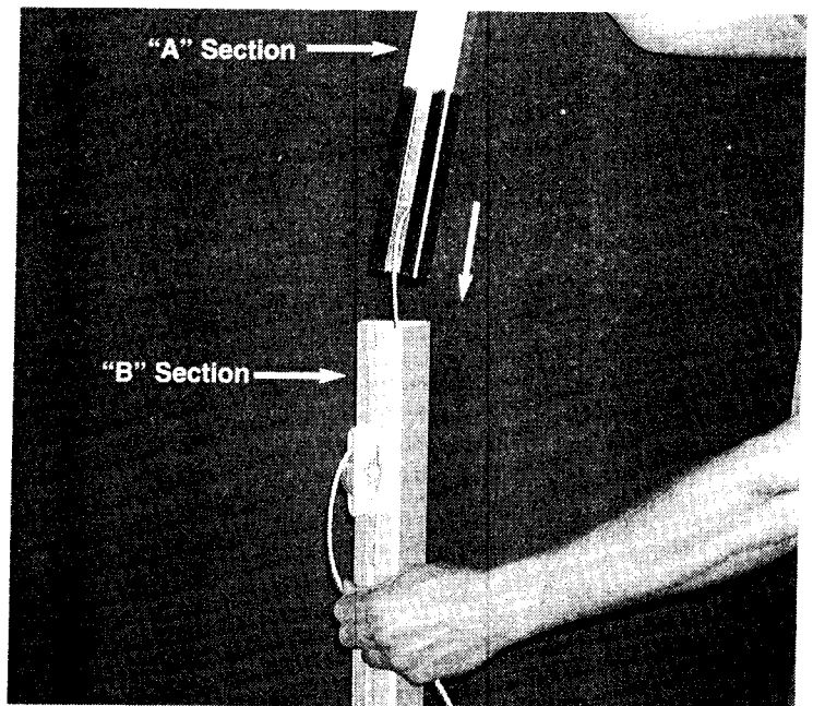
20. Pull the slack out of the cable and slide the "A" section into the "B" section. In the case of the extension 186-00, slide the "E" section into the "F" section.
