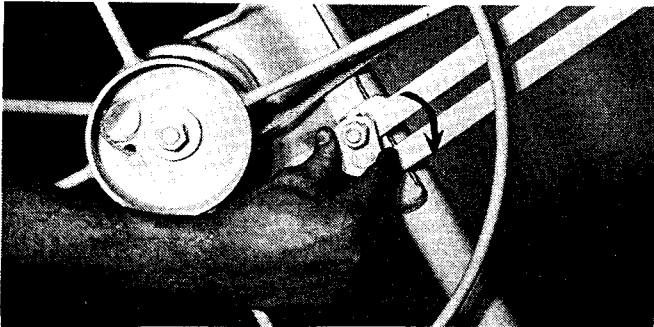
7. Now push the winch assembly back towards the frame. This action will automatically engage the slide bar lock. ALWAYS check to make sure that the slide bar lock is fully engaged by rotating it clockwise as far as possible before proceeding. The illustration shows a fully engaged slide bar lock. NOTE: DO NOT tighten the slide bar lock nut assembly. This will make it impossible to collapse the PANELLIFT® properly for transport and storage.
