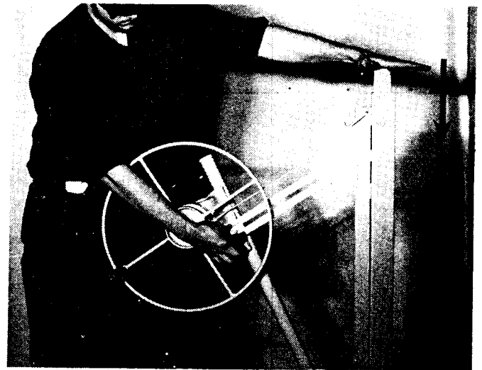
6. While holding the slide bar lock in this disengaged position with your right hand, push down on top of the telescoping section with your left hand. This action will cause the winch assembly to move toward the frame.
