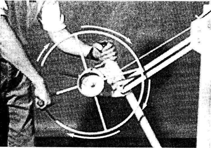
25. Rotate the winch in the direction shown to take the slack out of the cable.
