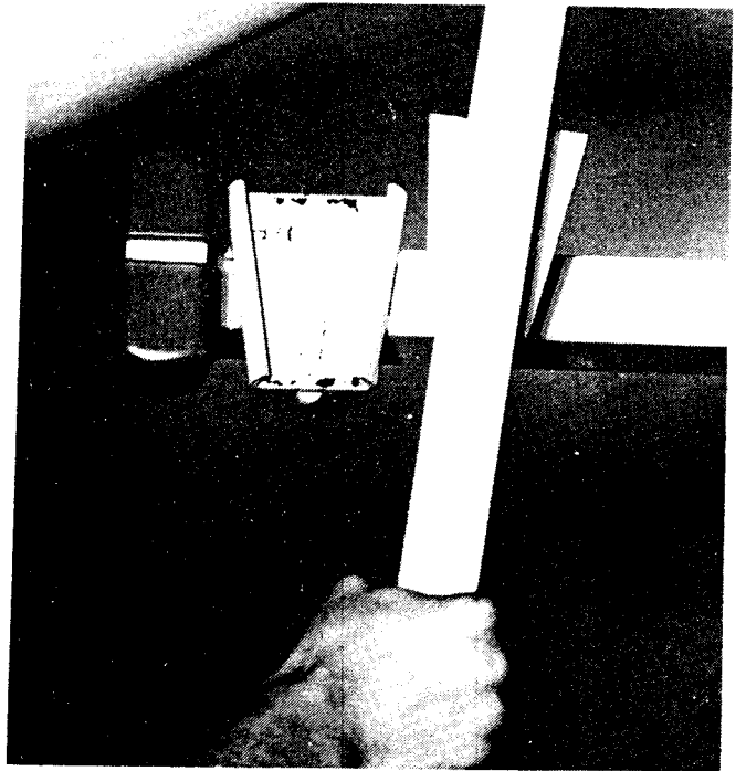
9. Place the tapered plates of the crossarms into the tapered sockets on the cradle. The spring tab on the back of the crossarm will lock it into place.
