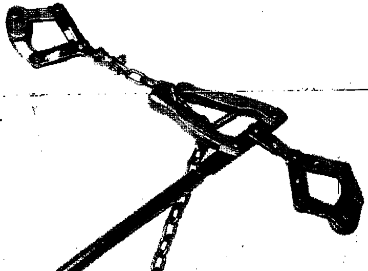
Figure 1. Joining wire in the middle of a strain.
