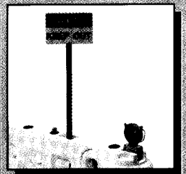
Pivot section supplied in Safety Orange and White - allows angle adjustment up to 75°.
