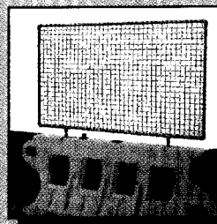
Moulded recesses in barrier provide for fixing of crowd control and security fences, signage and warning lights.
