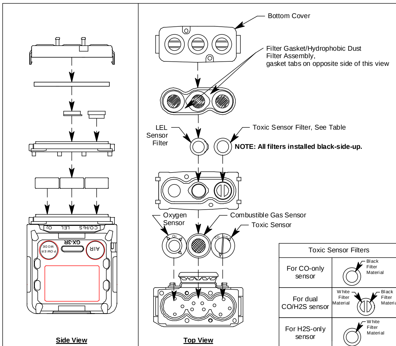
Figure 15: Replacing a Sensor
