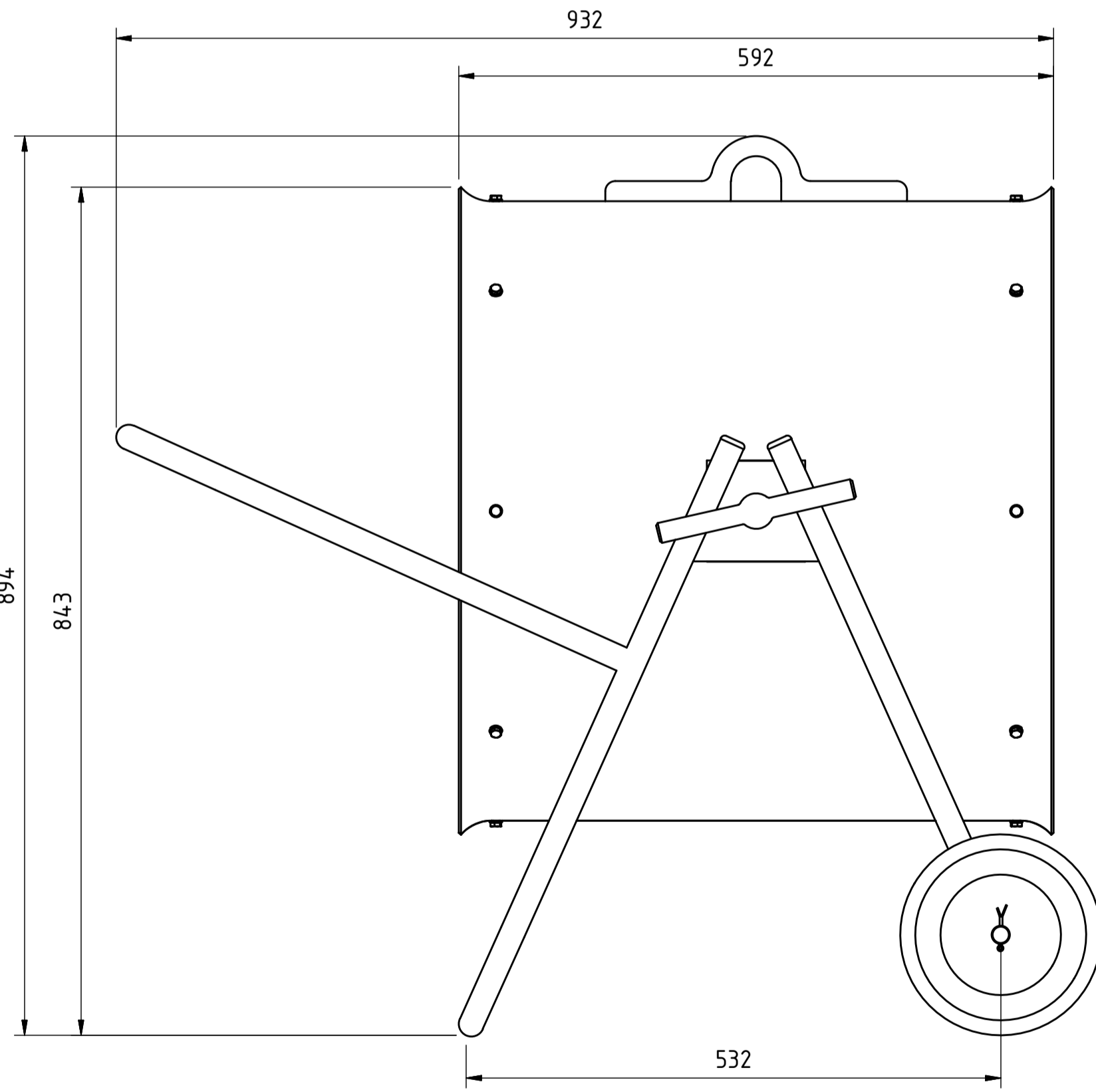
600mm MANCOOLER FAN PART No. - 200953 SCALE - 1 : 5
