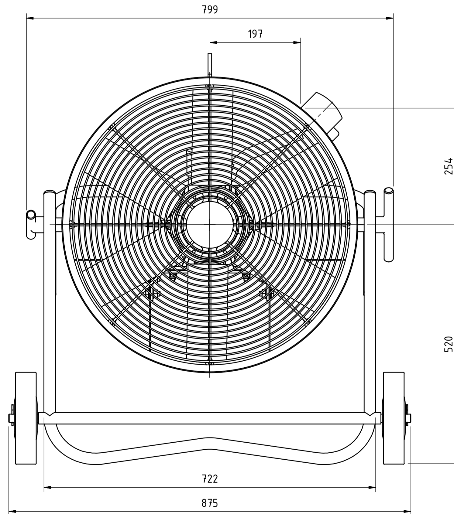
PICTORIAL VIEW PART No. - 200953 (BARREL NOT SHOWN) SCALE - 1 : 5
